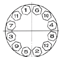
12 Bolt Pattern
