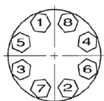
8 Bolt Pattern
